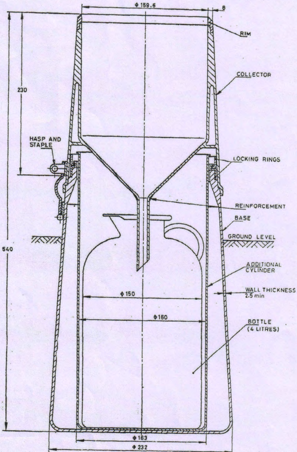
All dimensions in millimetres. RAINGAUGE, NON-RECORDING ( 200 cm 2 ), GENERAL ASSEMBLY
